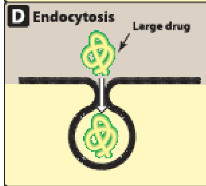
Figure 1.6 Schematic representation of drugs crossing a cell membrane. ATP = adenosine triphosphate; ADP = adenosine diphosphate.
